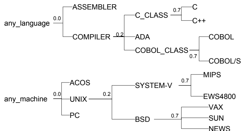
Figure 4. Examples of Abstraction Hierarchies, after Kitano & Shimazu, [14]
