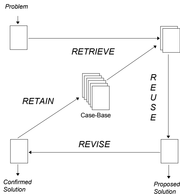
Figure 1 The CBR-cycle after Aamodt & Plaza [6]
