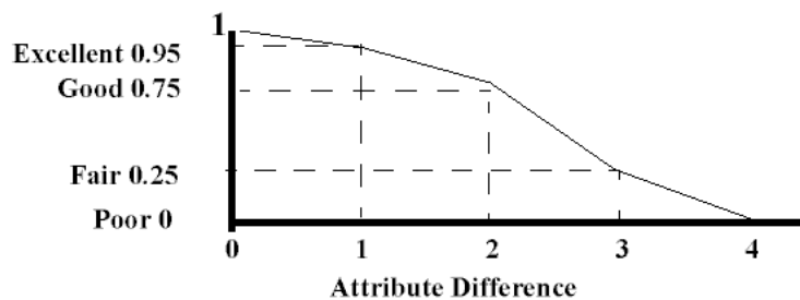
Fig. 3. A Fuzzy Preference Function, after Cheetham & Graf, [13]
